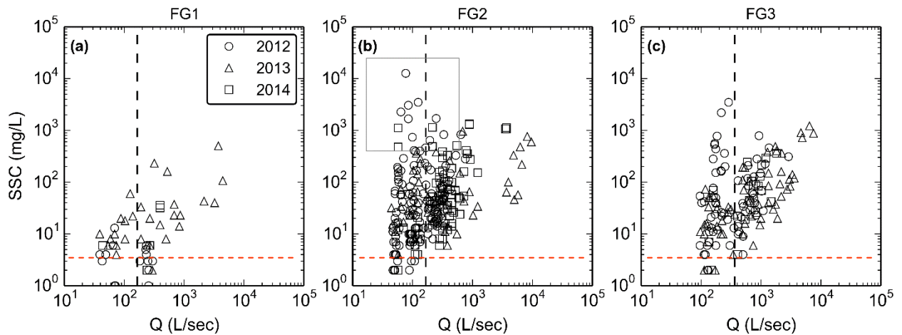
Figure 9. Discharge (Q) versus suspended sediment concentration (SSC) at the (a) forest, (b) quarry, and (c) village sites. The box in (b) highlights where SSC was high during low streamflow, downstream of the quarry, and then slightly diluted downstream near the hospital (c). These were notably absent from the forest site (a), and are hypothesized to be caused by activities at the quarry that ceased after 2012, i.e. washing sediment from the crushed aggregate during non-storm periods, and remediation of groundwater flow eroding sediment from haul surfaces. Red lines indicate the EPA fresh surface water quality standard: average Total Suspended Solids (comparable to SSC) not to exceed 5 mg/L. Vertical dashed lines indicate the threshold for defining stormflow. Discharge above the threshold is defined as stormflow and discharge below the threshold is defined as baseflow. Note that some samples collected under baseflow conditions occurred after rainfall but did not cause sufficient rise in stage to be defined as stormflow.
