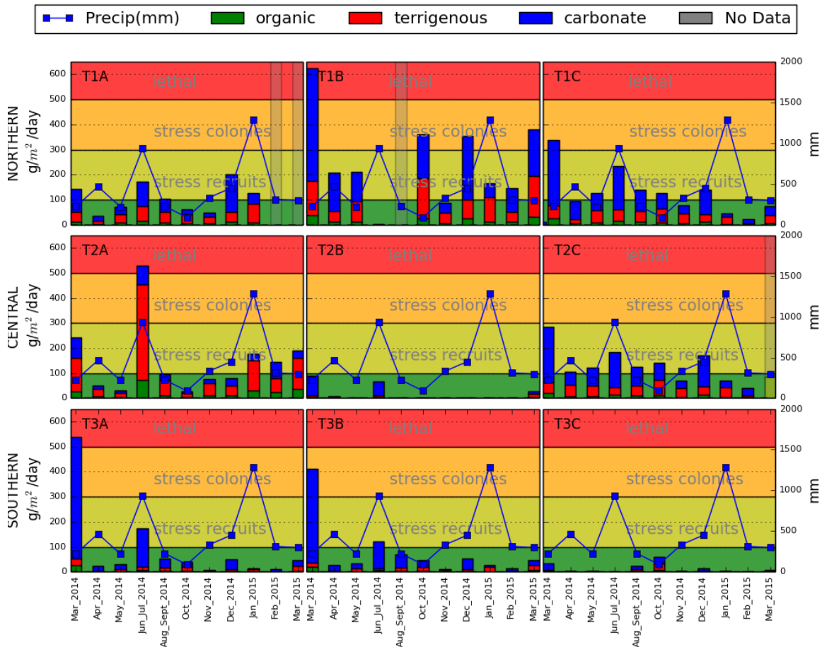
Figure 12. Time series of sediment accumulation in the tubes, March 2014-March 2015. Thresholds vary by coral species but most sources agree sedimentation rates over 500 g/m 2 /day are usually lethal (Ertemeijer et al., 2012; Fabricius, 2005).
