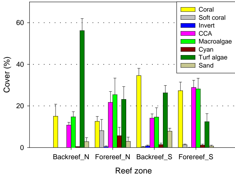
Figure 15. Spatial comparison of mean benthic percent cover of shallow habitats of the northern and southern backreef and forereef areas in Faga’alu Bay, American Samoa, derived from line-point-intercept surveys conducted in March 2012 and August 2013.
