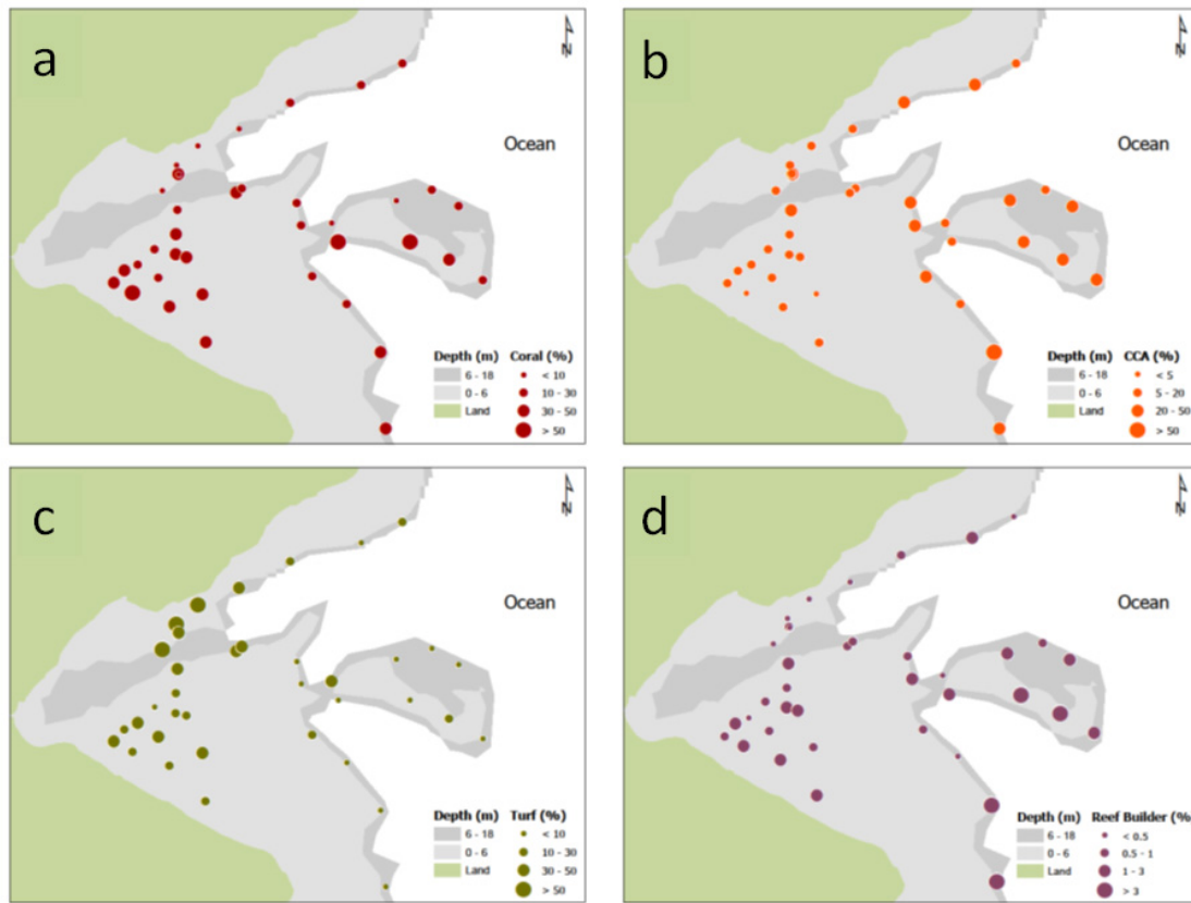
Figure 16. Spatial comparison of mean cover (%) values for (a) live hard corals, (b) crustose coralline algae (CCA), (c) turf algae, and (d) values of the reef-builder ratio (ratio of mean cover for corals and crustose coralline algae combined to cover for non-accreting organisms) from line-point-intercept surveys conducted in March 2012 and August 2013 in Faga'alu Bay.
