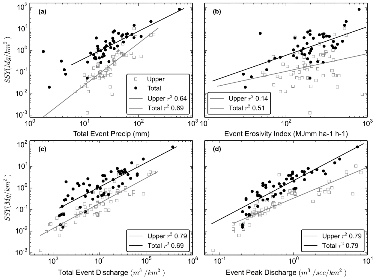
Figure 10. Storm event sediment yield (tons/km 2 ) from the upper watershed (undisturbed forest, FG1 in Figure 8), and from the total watershed (including the quarry and village, FG3 in Figure 8), versus (a) rainfall, (b) rainfall erosivity, (c) event discharge, and (d) event peak discharge. Each point represents the SSY for a single storm event. SSY for the disturbed watershed is higher than for undisturbed upper watershed, indicating human disturbance in the quarry and village has increased SSY EV above natural levels. Qpeak (d) showed the best model fit ( r^2 = 0.79 ) for both the Upper and Total watersheds. This model can be used to predict pre-mitigation SSY and compare to post-mitigation SSY, illustrating the effectiveness of mitigation. By reducing SSY through mitigation at the quarry, SSY measured during storms post-mitigation should plot on the model for the upper watershed, indicating SSY from the watershed is back to the natural baseline SSY
