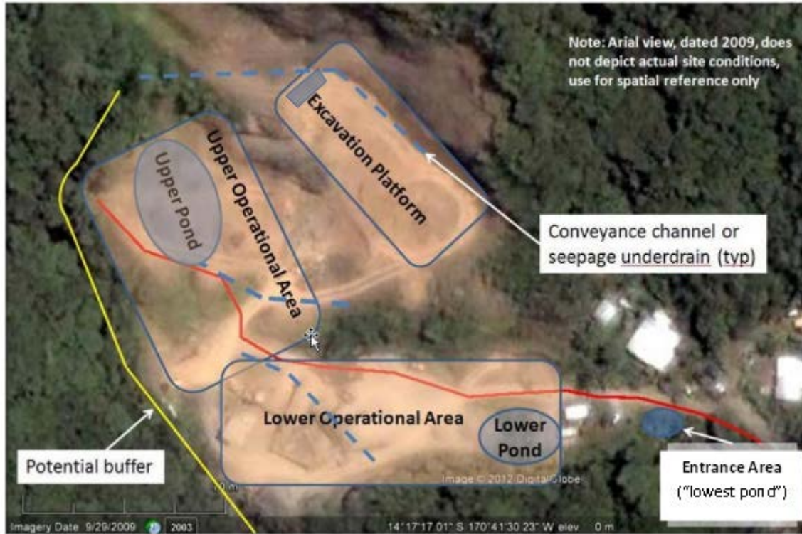
Figure 3. Schematic of retention pond locations at the Samoa Maritime quarry (Horsley Witten Group Inc., 2013). The “conveyance channel/seepage underdrains” (dotted blue lines) were constructed in 2012. Actual locations may vary slightly from this diagram. The underdrain through the Lower Operational Area was routed east of the Lower Pond towards the Entrance Area. The “potential buffer” was installed with the retention ponds in 2014. The “lowest pond” was present in 2012, but reconstructed in 2014 to increase its effectiveness.
