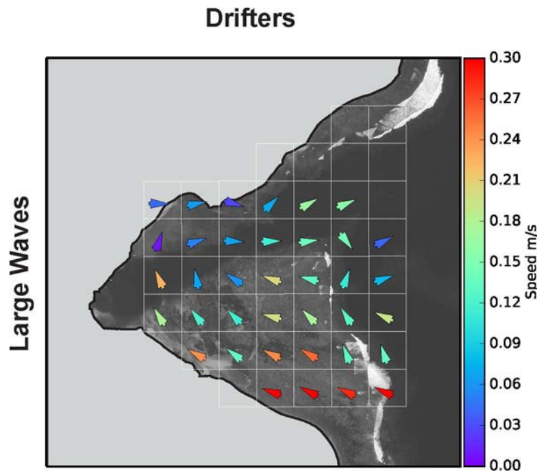
Figure 2. Gridded mean current speeds and directions for 100 m 2 grid cells based on GPS-drifter data. Current speeds are highest, and directions less variable during large waves and high winds. Current speeds are slower, and directions more variable during small waves and light winds (Messina, Storlazzi, Biggs, et al., n.d.).
