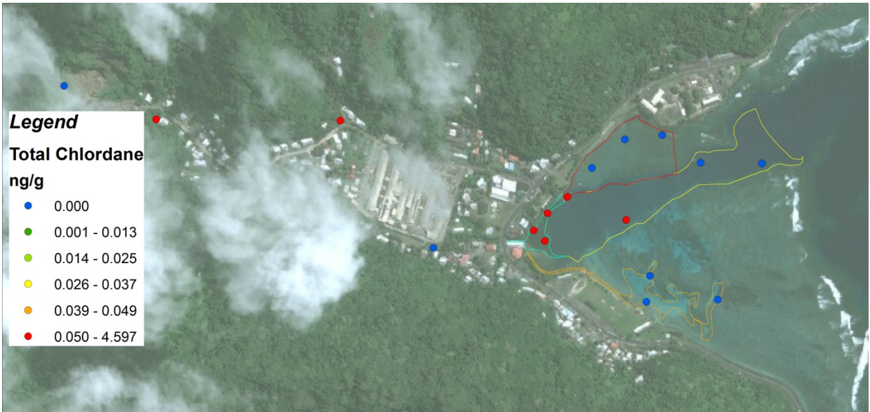
Figure 19. Total chlordane concentrations in sediments (January, 2014). This is a representative figure showing a strong watershed pollutant source.
