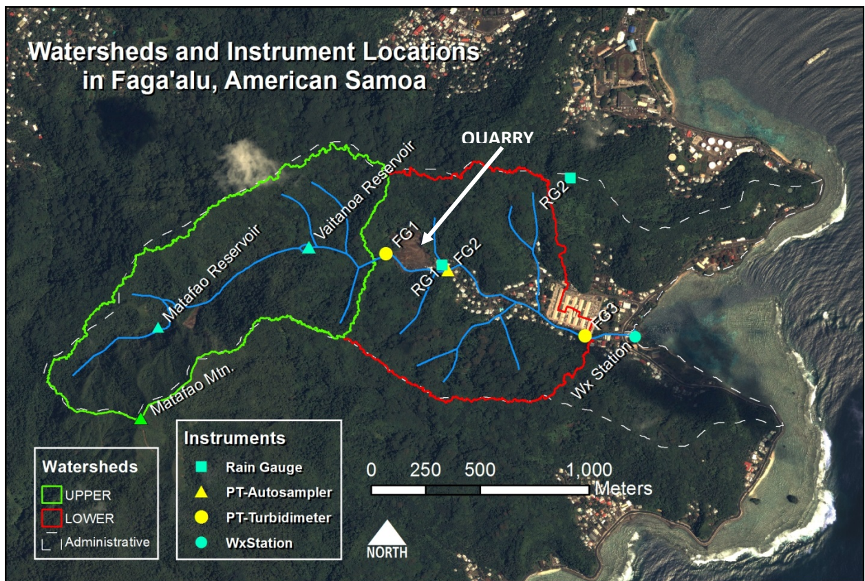
Figure 8. Location map of monitoring sites at Faga'alu. "Wx station" is a weather station with a rain gauge, wind speed, and air pressure.
