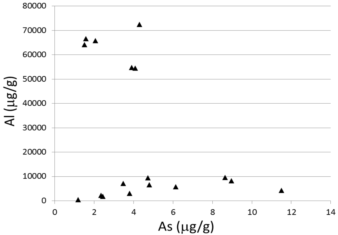
Figure 22. Scatter plot of sediment Arsenic (As) versus sediment Aluminum (Al). The lack of correlation between these two crustal elements suggests that high arsenic levels are likely due to anthropogenic sources.
