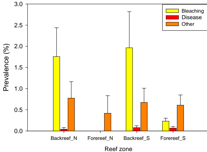
Figure 18. Spatial comparison of prevalence (%) of bleaching and disease from belt-transect surveys conducted in March 2012 and August 2013 in Faga’alu Bay.
