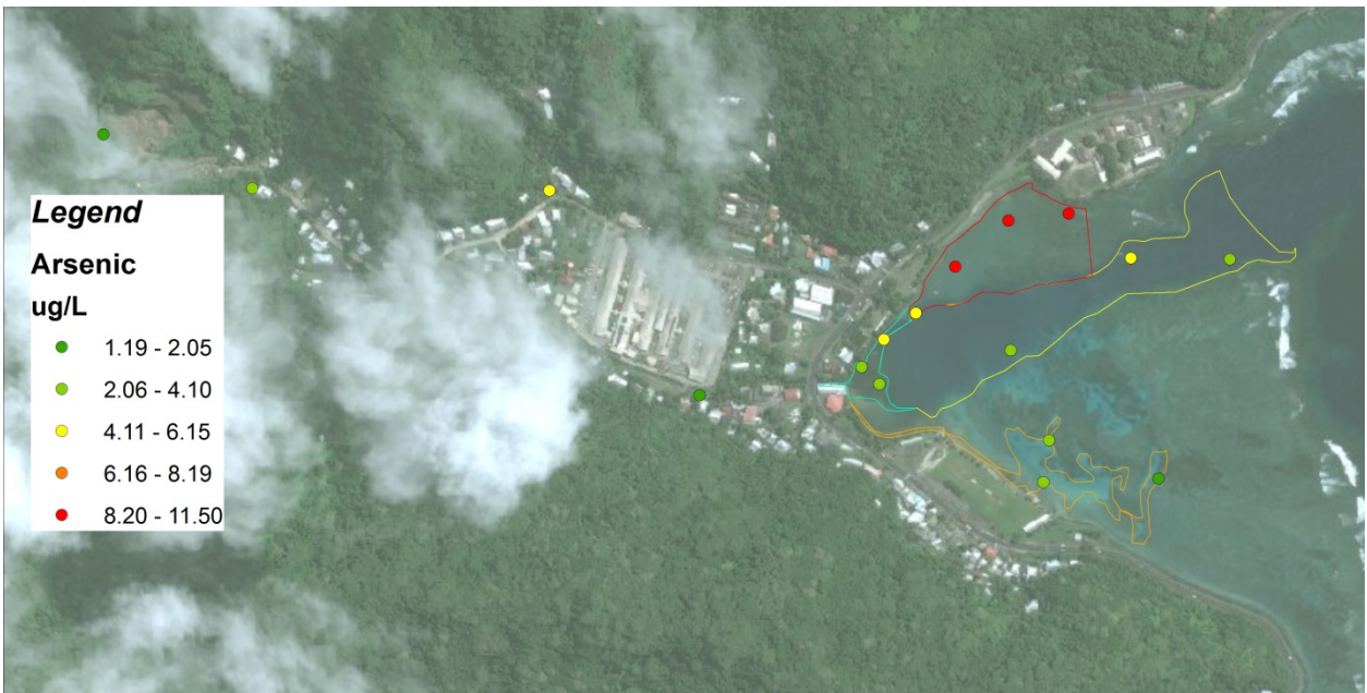
Figure 20. Arsenic concentrations in sediments (January, 2014). Note: highest concentration are in the North Bay area.
