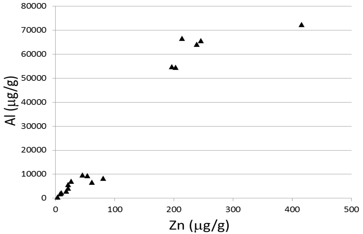
Figure 21. Scatter plot of sediment Zinc (Zn) versus sediment Aluminum (Al). The high degree of correlation between these two crustal elements (Spearman rho=0.96) suggests that even though Zn exists at high levels, this is most likely naturally occurring Zn.
