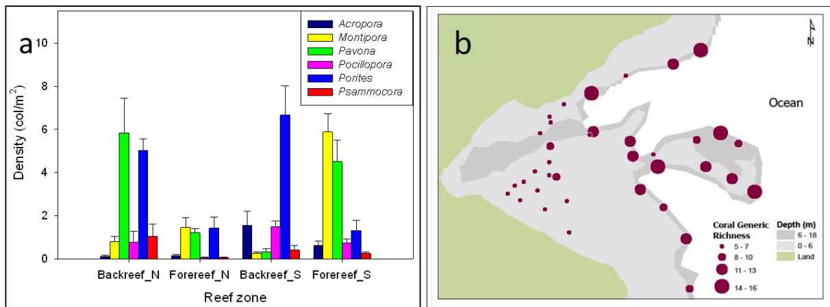
Figure 17. Spatial comparison of (a) coral-colony density (colonies/m 2 ) and (b) total coral generic richness from belt-transect surveys conducted in March 2012 and August 2013 in Fagaʻalu Bay. The color-coded bars indicate densities of selected dominant coral genera
