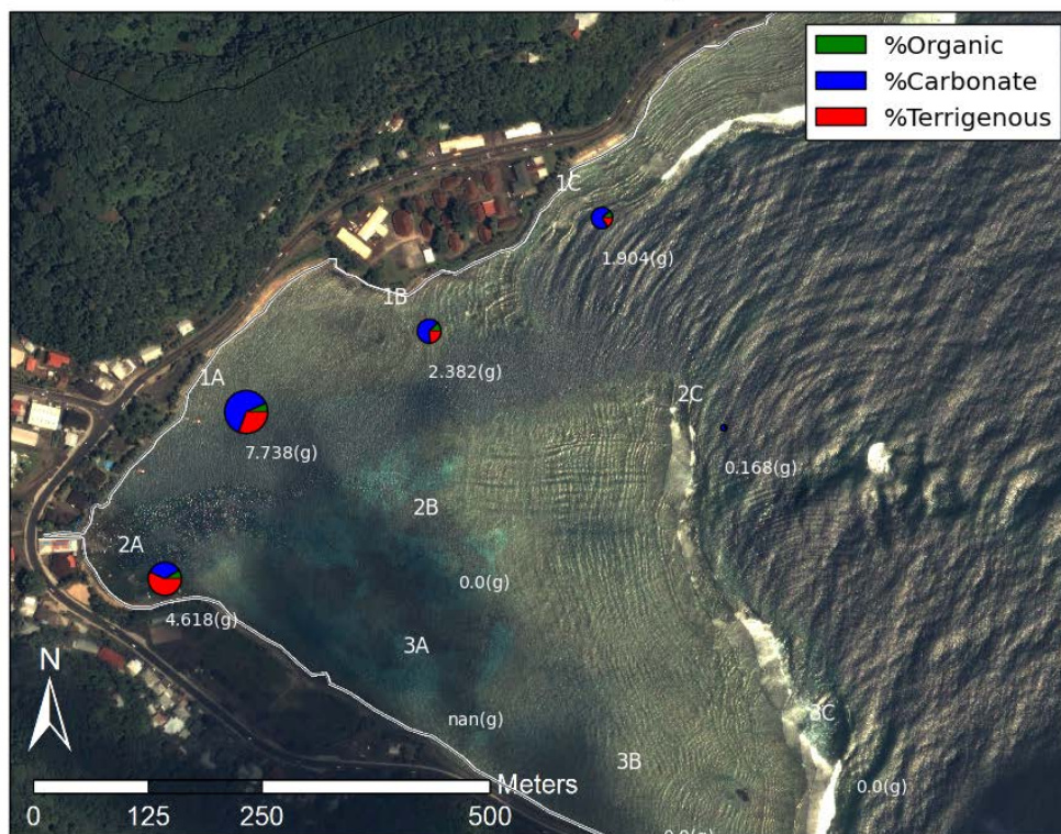
Figure 11. Map showing locations of co-located SedPods and tubes, and sample plots with amounts (circle size) and the organic, carbonate and terrestrial fractions, for one month of sedimentation in April 2014. Similar data was collected April 2014-April 2015 but not presented here.
