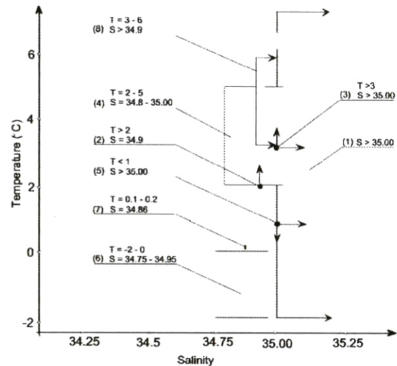
Figure 2. The temperature–salinity characteristics of the Barents Sea Atlantic Water (AW).
