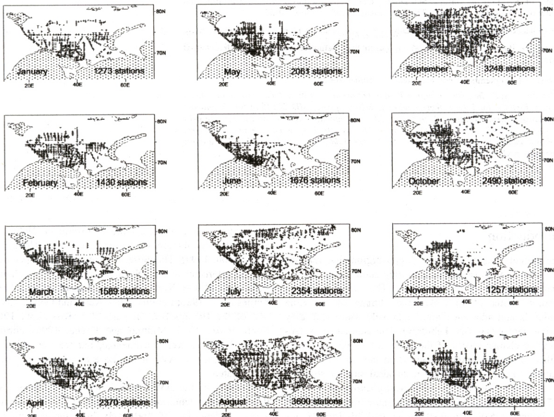
Figure 1. Oceanographic-station locations in the Barents Sea from 1900 to 1990.
