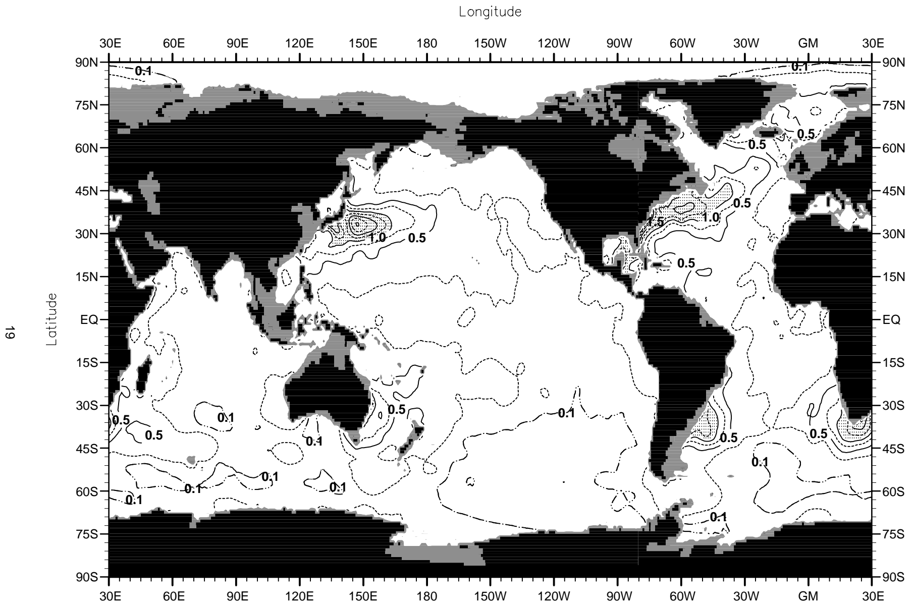
Fig. 14 Interannual std. deviation of seasonal mean temperature ( ^{\circ}\text{C} ) anomaly fields for 1948-98 at 500 m depth. Solid contours represent intervals of 0.5^{\circ}\text{C} and dashed lines represent intervals of 0.25 .
