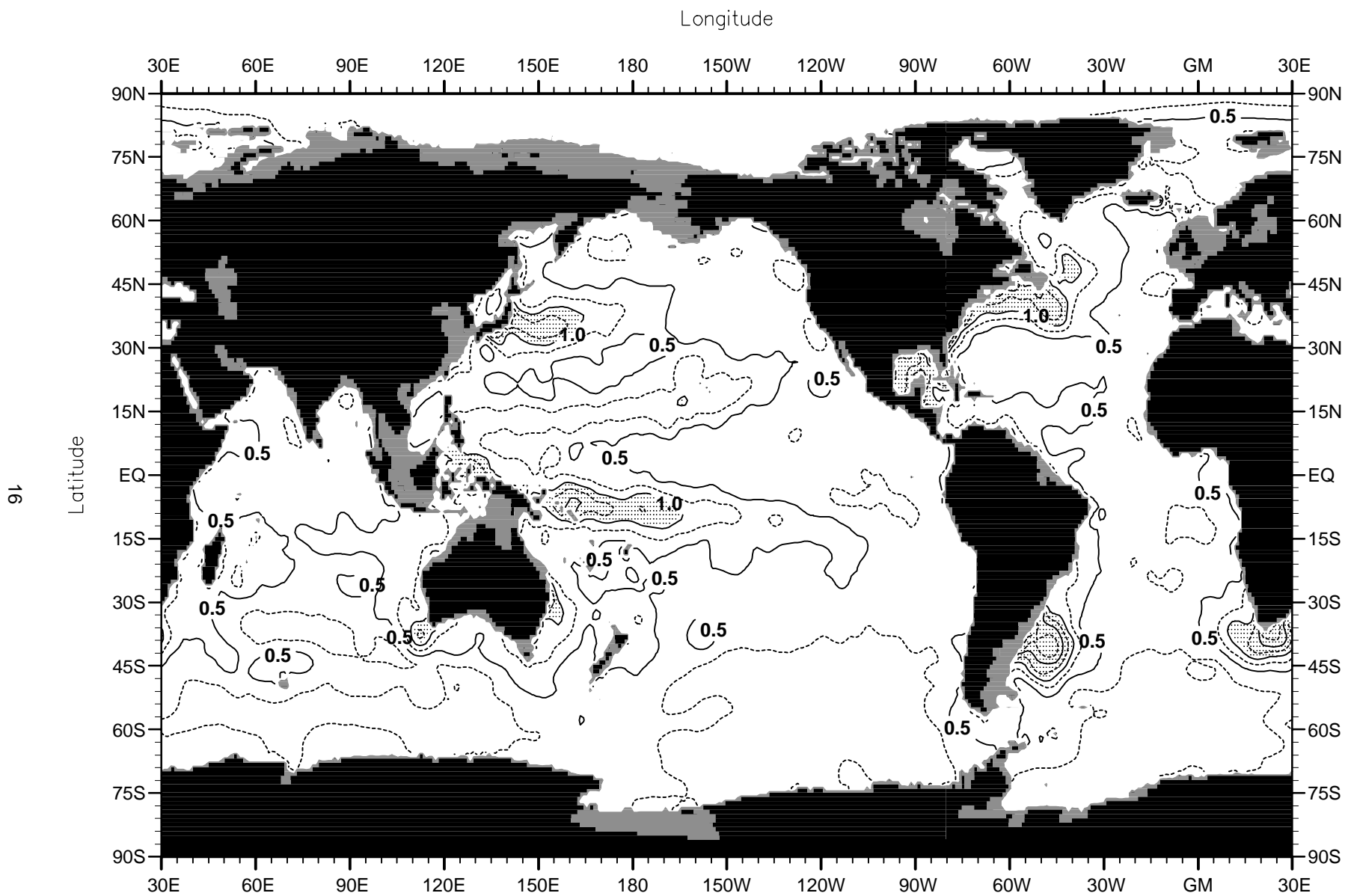
Fig. 11 Interannual std. deviation of seasonal mean temperature ( ^{\circ}\text{C} ) anomaly fields for 1948-98 at 250 m depth. Solid contours represent intervals of 0.5^{\circ}\text{C} and dashed lines represent intervals of 0.25 .
