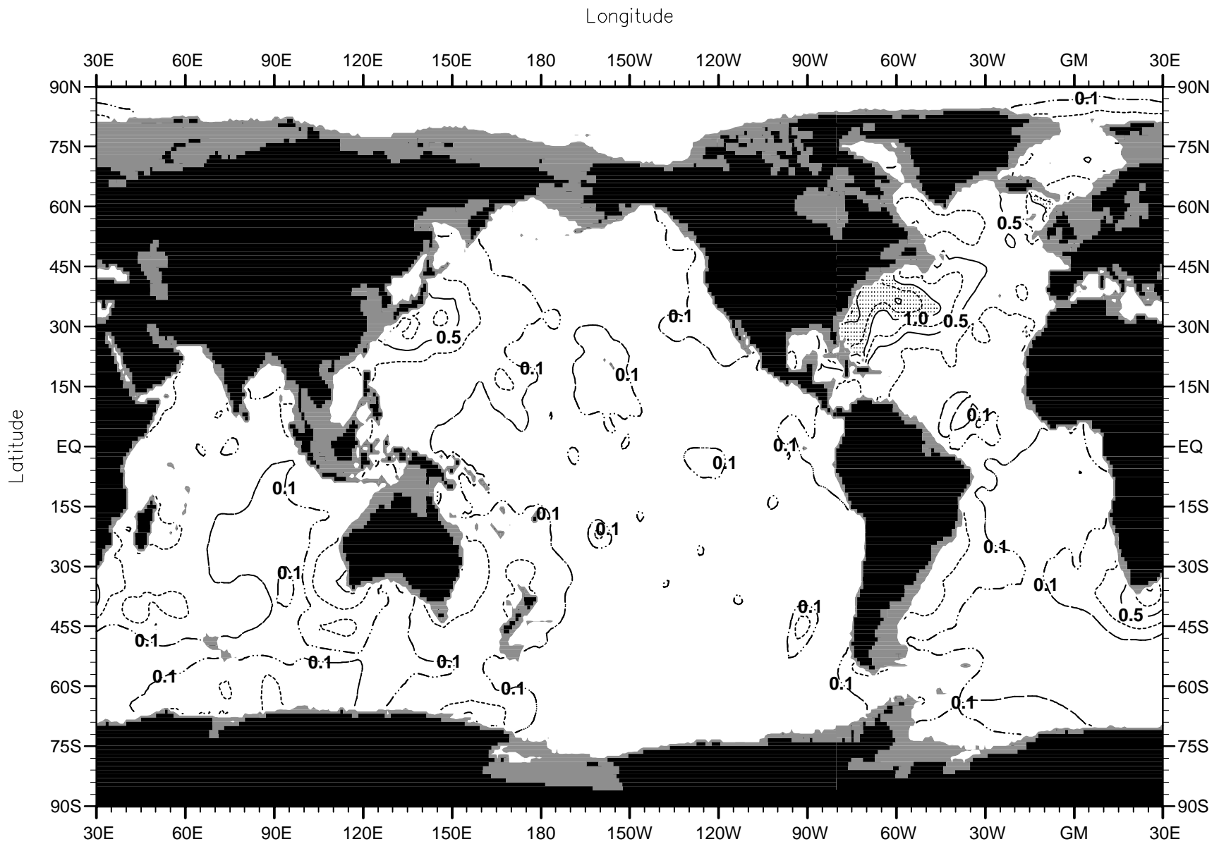
Fig. 17 Interannual std. deviation of seasonal mean temperature ( ^{\circ}\text{C} ) anomaly fields for 1948-98 at 800 m depth. Solid contours represent intervals of 0.5^{\circ}\text{C} and dashed lines represent intervals of 0.25 .
