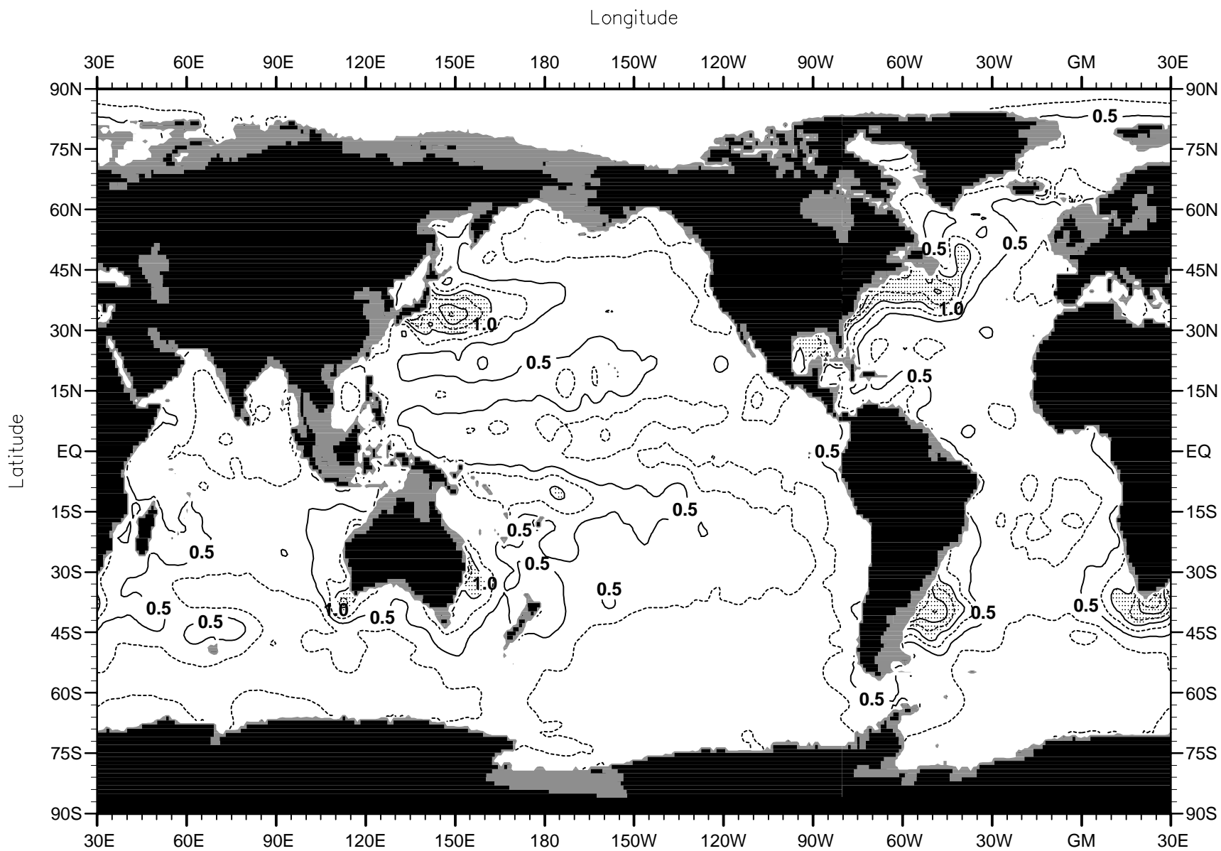
Fig. 12 Interannual std. deviation of seasonal mean temperature ( ^{\circ}\text{C} ) anomaly fields for 1948-98 at 300 m depth. Solid contours represent intervals of 0.5^{\circ}\text{C} and dashed lines represent intervals of 0.25 .
