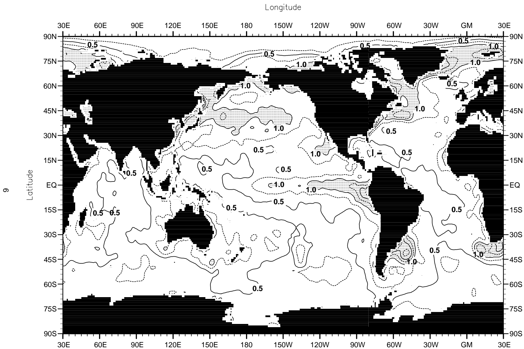
Fig. 1 Interannual std. deviation of seasonal mean temperature ( ^{\circ}\text{C} ) anomaly fields for 1948-98 at the sea surface. Solid contours represent intervals of 0.5^{\circ}\text{C} and dashed lines represent intervals of 0.25 .
