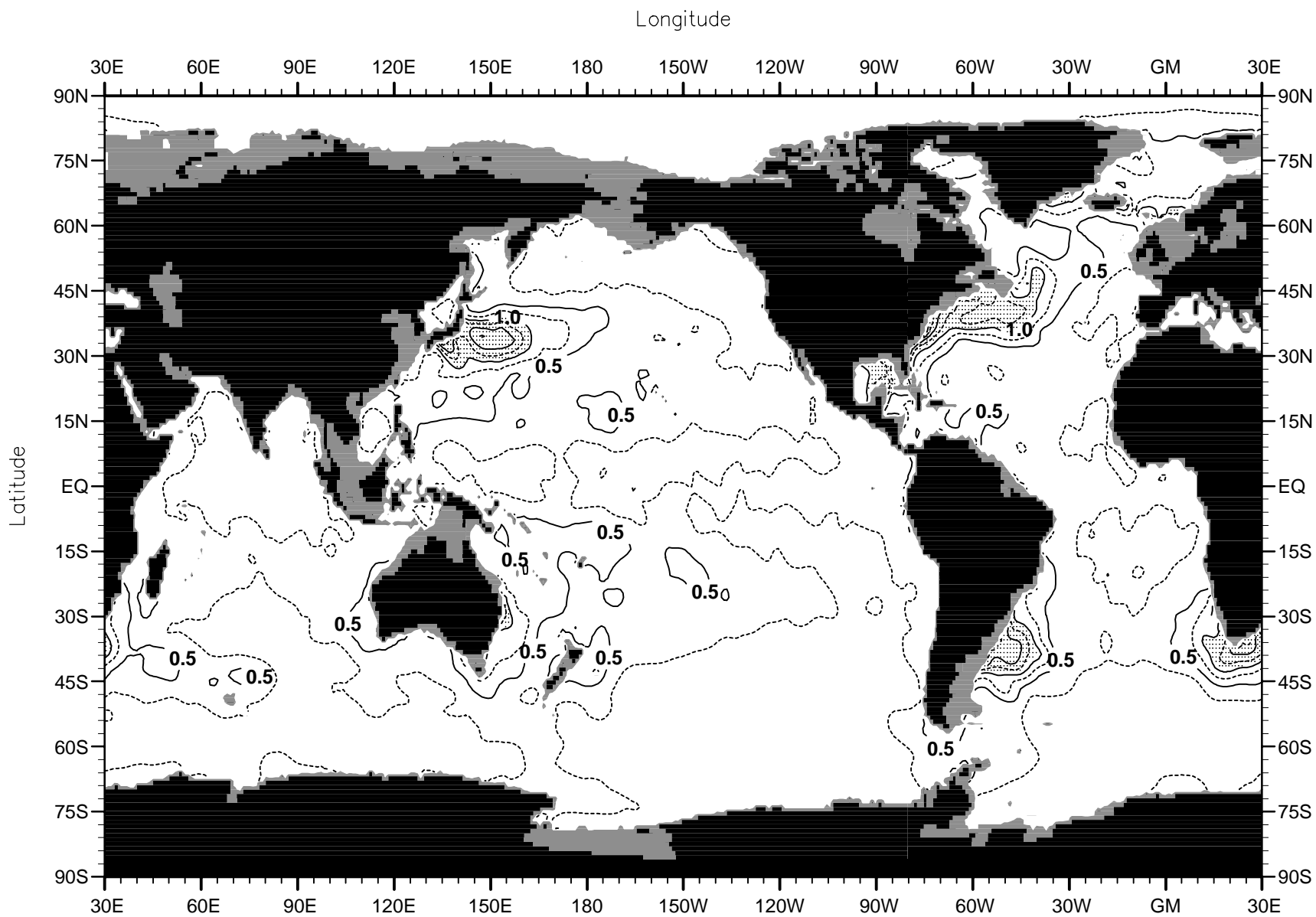
Fig. 13 Interannual std. deviation of seasonal mean temperature ( ^{\circ}\text{C} ) anomaly fields for 1948-98 at 400 m depth. Solid contours represent intervals of 0.5^{\circ}\text{C} and dashed lines represent intervals of 0.25 .
