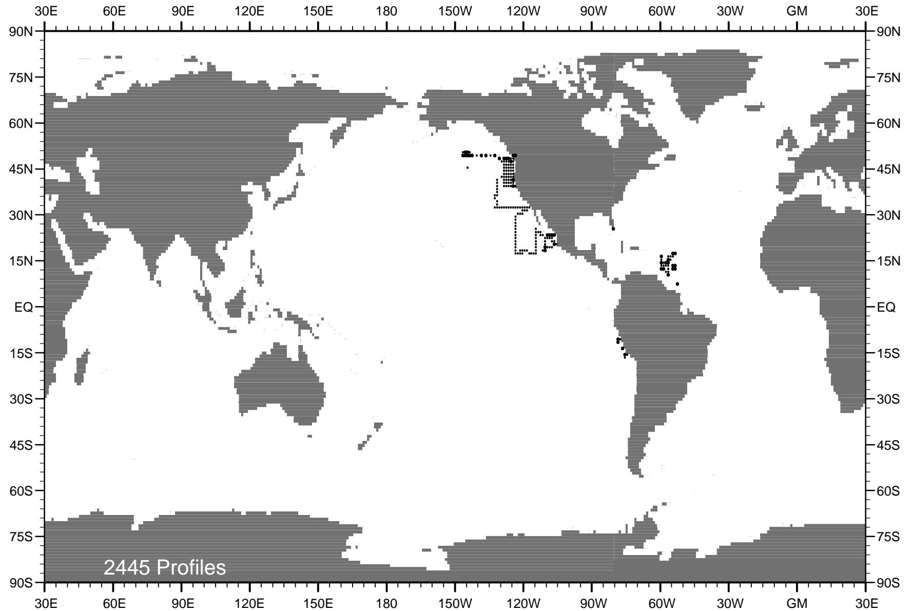
Fig. A3 WOD01 CTD cast distribution for year 1969 .
