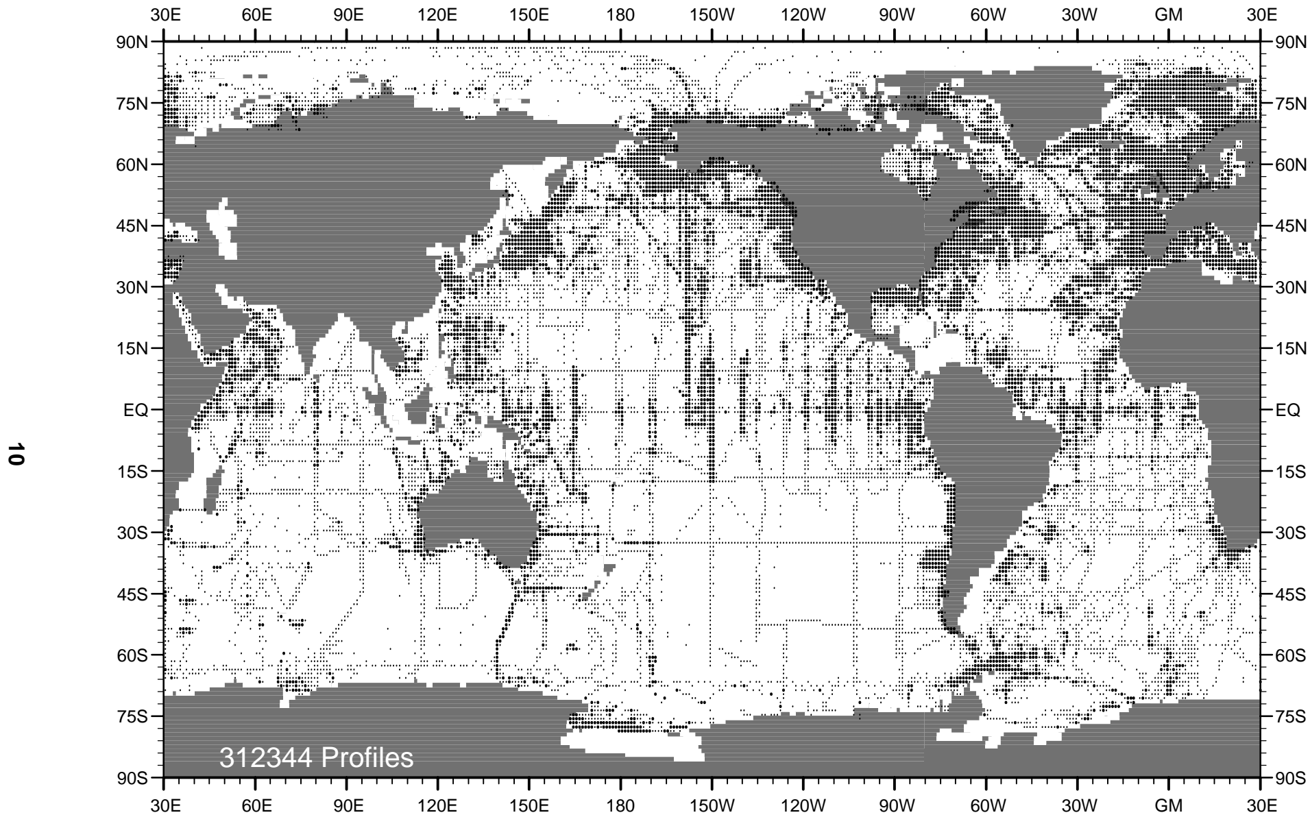
Fig. 4 Distribution of all casts in the CTD files of WOD01. Dots show location of 1-degree squares containing any data.
